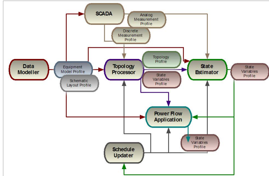
Figure 6-5 EMS Network Analysis Systems and Data Exchanges
