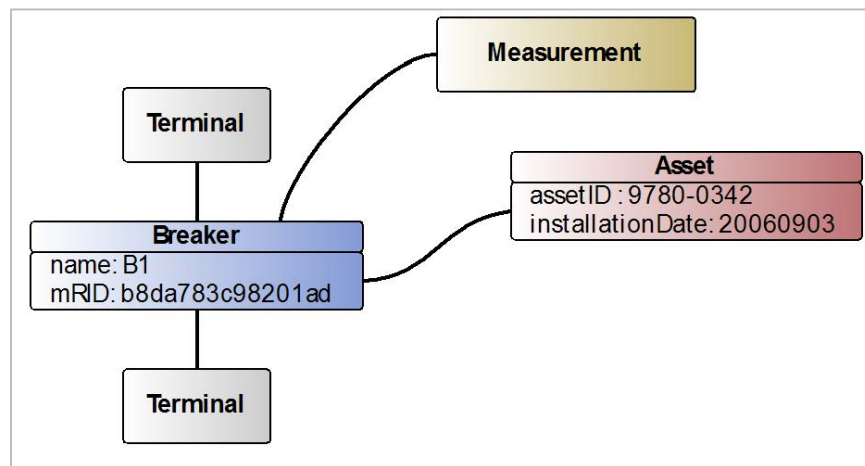
Figure 5-22 Breaker-Asset Instance Example
