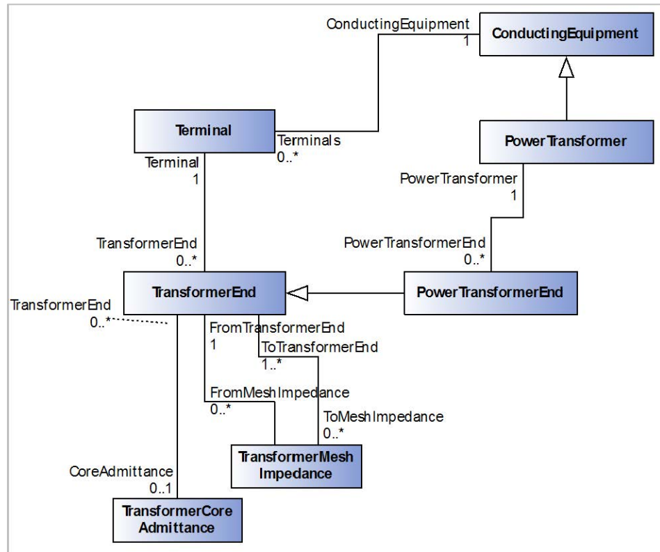
Figure 5-16 Balanced Power Transformer Classes
